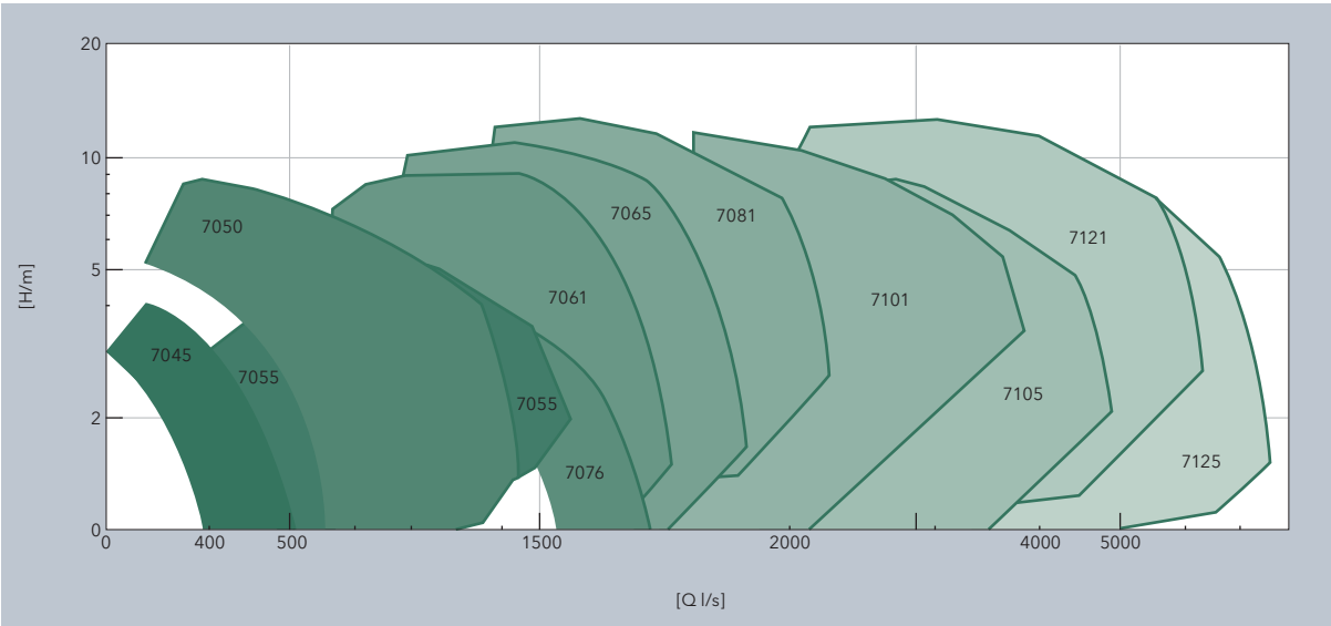
Performance range, 50 Hz
