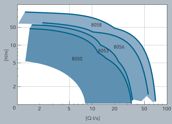
Performance (50 Hz)
